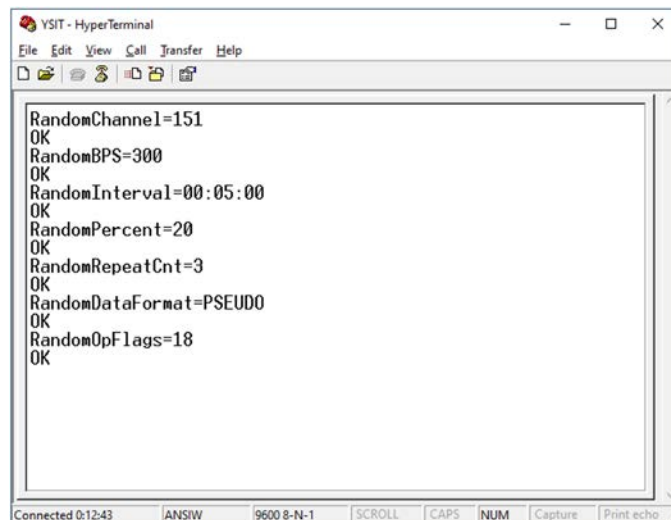
Figure 6 | Random Transmission Terminal Setup
